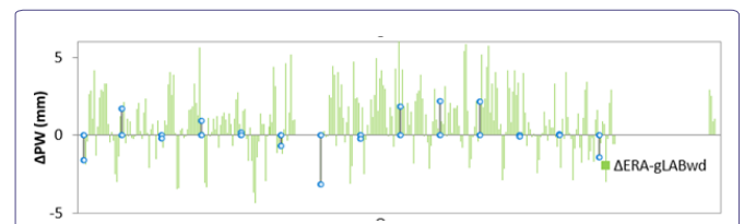
Figure 5: Trend and differences between global interpolated PW and gLAB computed PW weather dependent for site DODM with respect to time.
