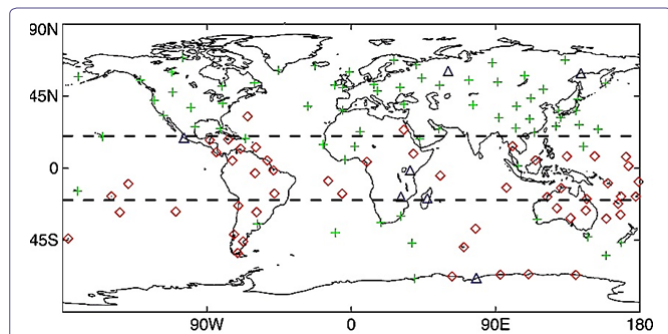
Figure 1: GUAN Ground based GPS stations as of February 2021 as recorded by ECMWF. Stations that contain both daytime and nighttime data are denoted by green crosses, whereas daytime-only stations are denoted by red diamonds, and nighttime-only stations are denoted by blue triangles.
