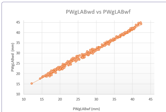
Figure 3B: The Correlation between gLAB computed PW weather dependent against the gLAB computed PW weather free. The computed Pearson correlation coefficient is 0.9967.
