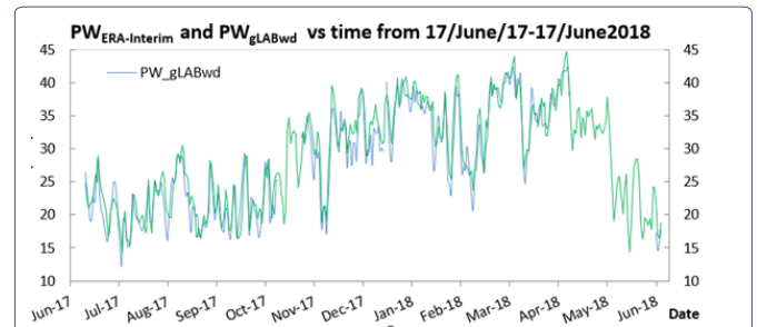
Figure 4: Comparison of global interpolated PW and gLAB computed PW weather dependent for site DODM . Blue is gLAB computed PW weather dependent and Green is global interpolated Pw from ERA-Interim.
