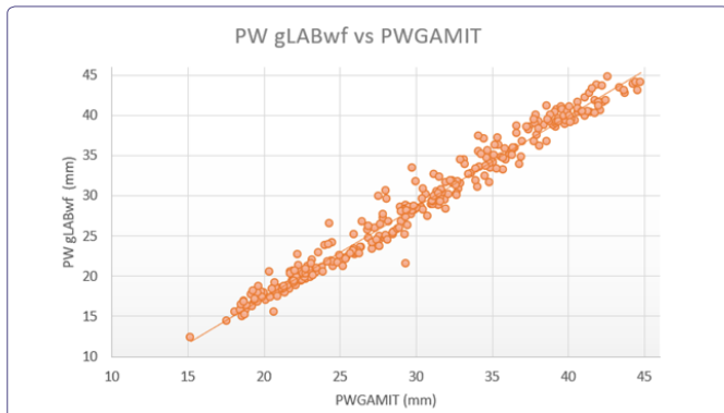
Figure 3A: The Correlation between gLAB computed PW weather free against the GAMIT computed PW. The computed Pearson correlation coefficient is 0.9867.
