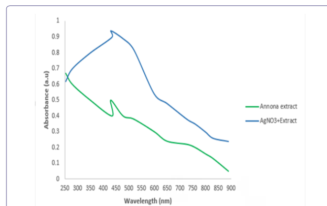
Figure 1: UV-visible absorption spectrum of silver nanoparticle produced.
