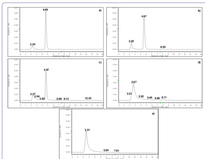
Figure 3: HPLC-DAD chromatograms of betamethasone subjected to stress conditions.
