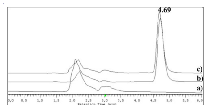
Figure 2: HPLC-DAD chromatograms to demonstrate the selectivity of the method.
