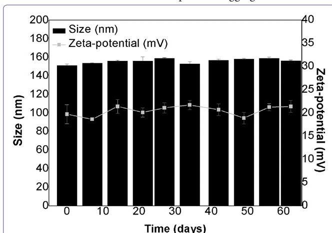
Figure 4: Evaluation of the liposomes stability. Size (nm; ■) and zeta-potential (mV; ■) obtained for LUVs entrapping betamethasone over a period of two months.
